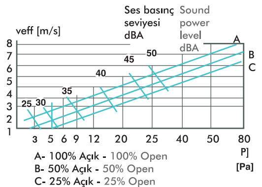
Zıt Kanatlı Damperli - With Opposed Blade Damper
