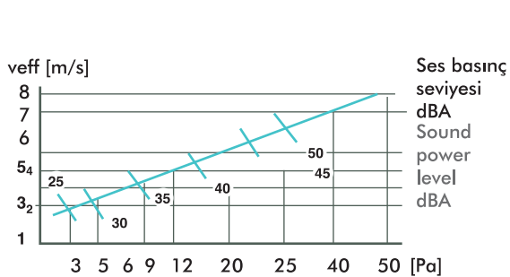
Dampersiz - Without Damper
