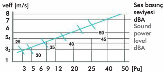
Dampersiz - Without Damper
