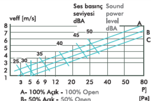
Zıt Kanatlı Damperli - With Opposed Blade Damper
